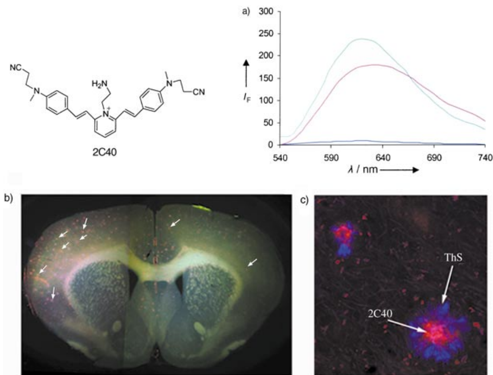
Figure 2. a) Fluorescence spectra of 2C40 (25 μM) with Aβ40 fibril (green line; 30 μL of a 0.5-mg mL -1 solution in PBS (pH 7.4) containing EDTA (1 mM)), and Aβ42 fibril (purple line; 30 μL of a 0.5-mg mL -1 solution in PBS solution (pH 7.4) containing EDTA (1 mM)) compared to a control buffer solution (dark blue line; 30 μL of a solution of PBS (pH 7.4) containing EDTA (1 mM)). b) Labeling of amyloid deposits with 2C40 in a slice of mouse brain (red, indicated by arrows). The image was taken with a charge-coupled device camera. c) Confocal microscopy image of amyloid deposits labeled with 2C40 (red) and ThS (blue); note that 2C40 preferentially labels the core of deposits.
